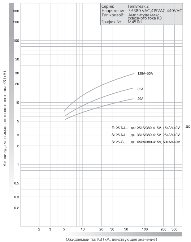
E125-NJ, S125-NJ, S125-GJ. 440V AC.
