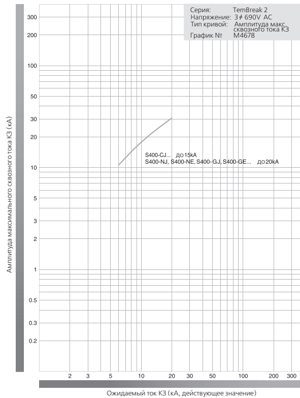
S400-CJ, S400-NJ, S400-NE, S400-GJ, S400-GE, 690V AC.
