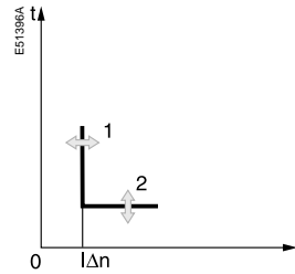
Micrologic 7.0 A
