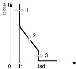
Micrologic 2.0 A
