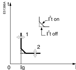
Micrologic 6.0 A
