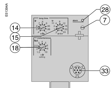
Micrologic 2.0 A
