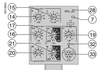
Micrologic 6.0 A
